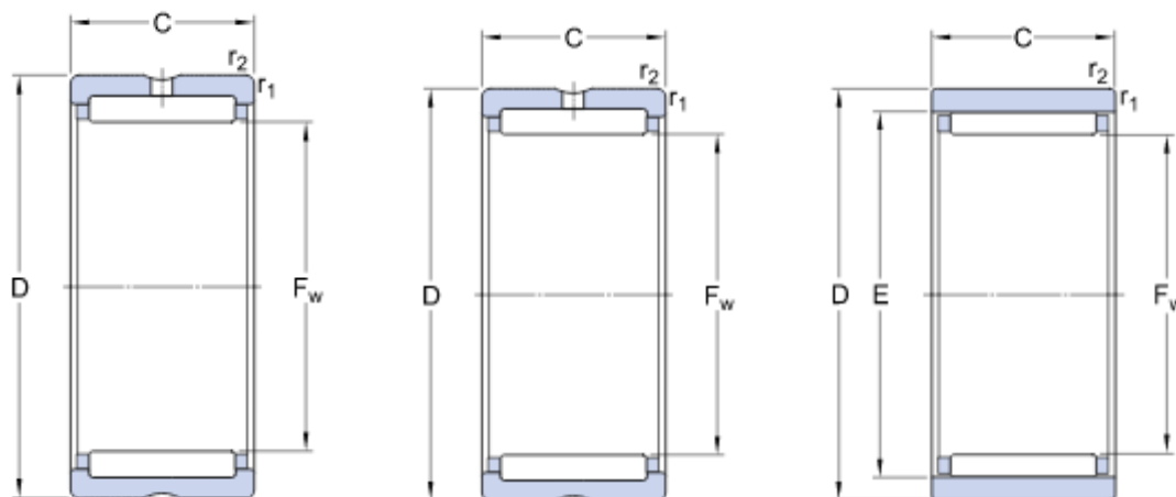
Needle Roller Bearing
