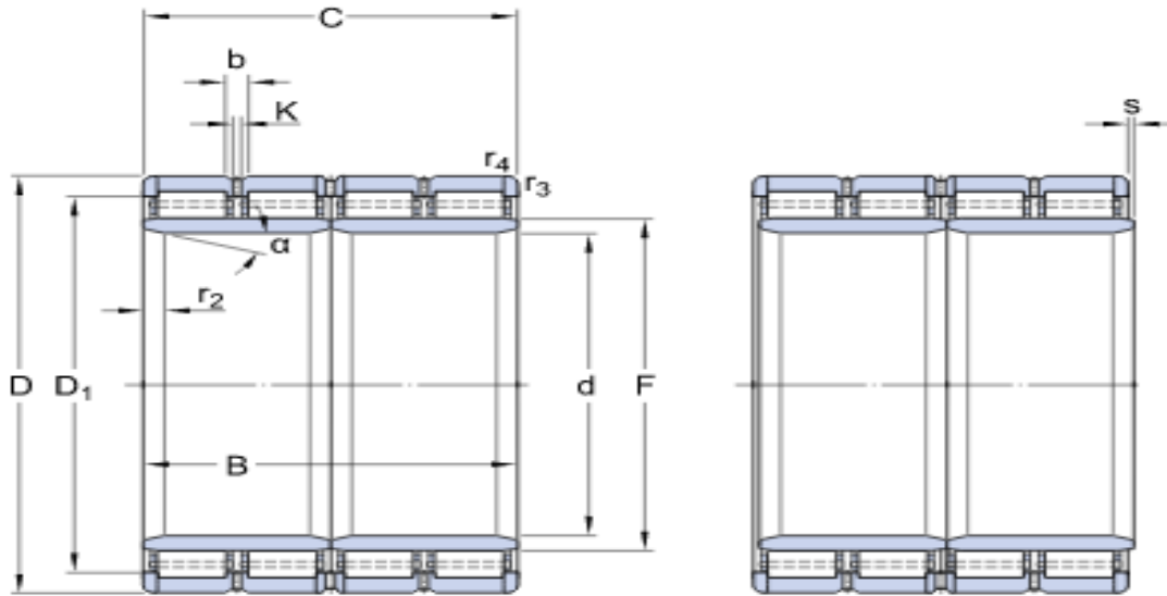
Four row Cylindrical Roller Bearing
