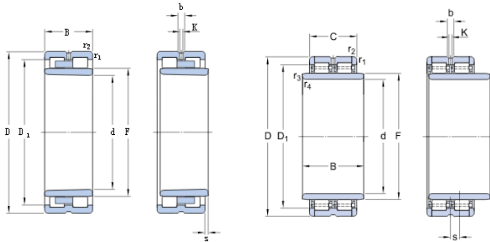
Double-row Cylindrical Roller Bearing
